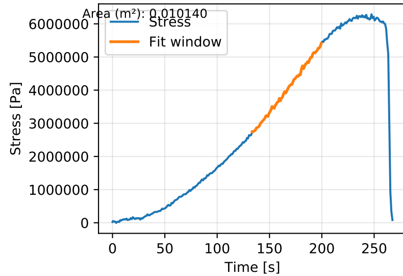
Stress vs Time
