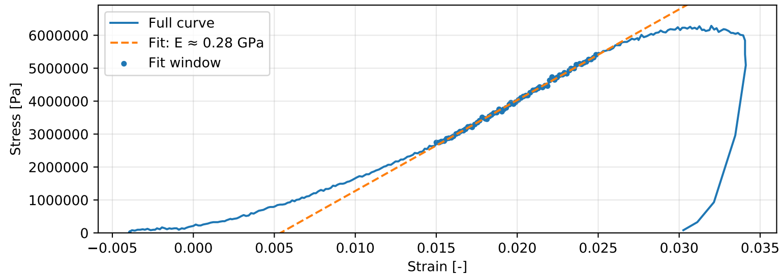
Stress vs Strain
